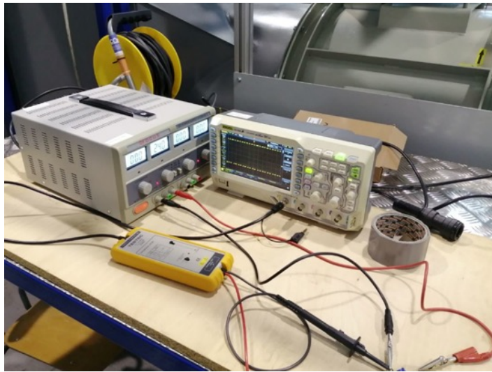
Segment of the experimental setup
