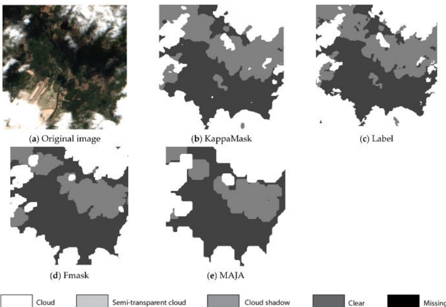
Comparison of LZA prediction output for a 512 × 512 pixels sub-tile in the test dataset. (a) Original Sentinel-2 True-Color Image; (b) KappaMask classification map; (c) Segmentation mask prepared by a human labeller; (d) Fmask classification map; (e) MAJA classification map.
