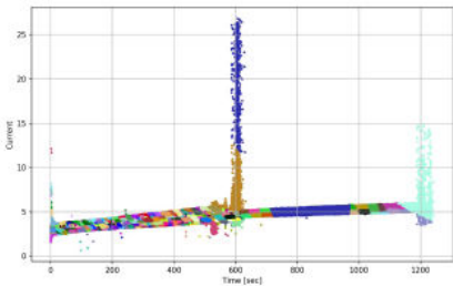
Figure 2: Partitioning of normal time series with minimum size 1000 into 362 partitions.
