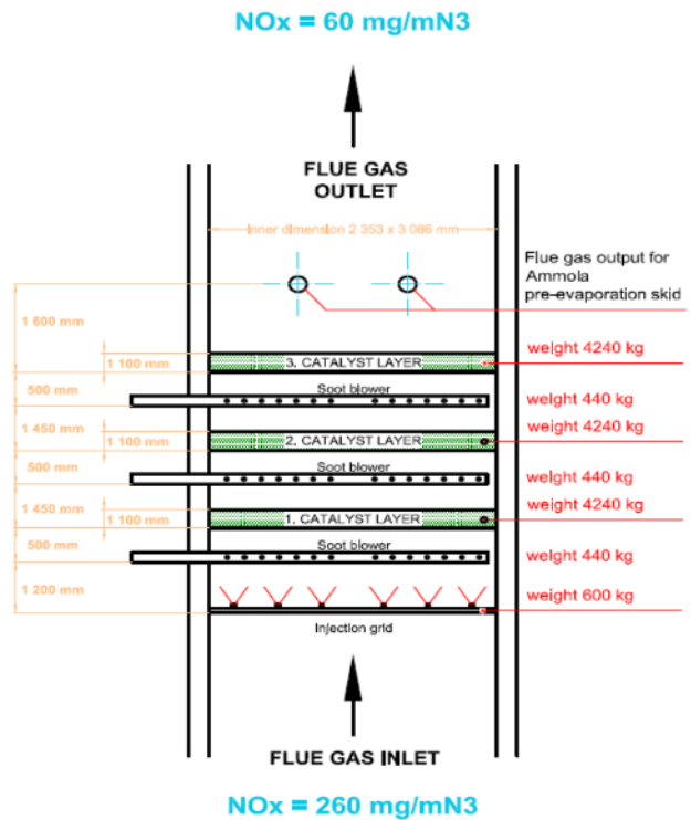
Basic sketch of the test reactor
