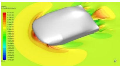
CFD simulation of the wave pattern of a trimaran
