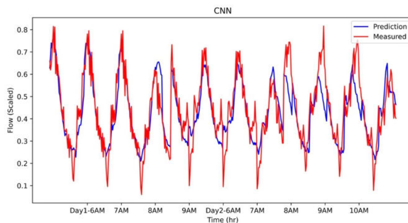
Result: The comparison of measured traffic at E4S for two consecutive days between 6 to 10 AM obtained from CNN (Convolutional Neural Network)
