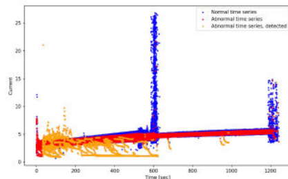
Figure 4: Display of abnormal points as detected by the algorithm. The identification of abnormal points are also possible within the areas covered by blue (normal) points. This is due to the modeling of slope and curvature
