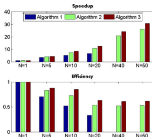
Figure 1: Speedup and efficiency of algorithms
