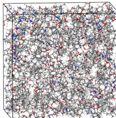
Figure 2: Simulation cell for the epoxy resin model with 90% crosslinking ratio by using 40 DETA and 100 DGEBA monomers.
