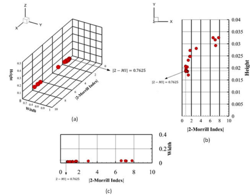
Figure 2. Variations of the parameters during optimisation. (a) Variations of width and height, variation of (b) height and (c) width.
