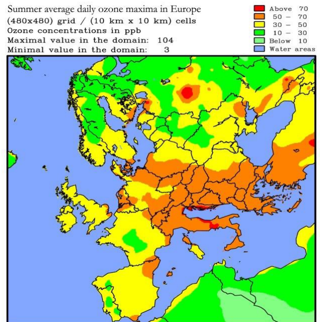
Summer average daily ozone maxima in Europe, calculated by the fine grid version of UNI-DEM (with 10x10 km. cells)
