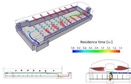
Figure 1. Tracing the glass particles inside the oven
