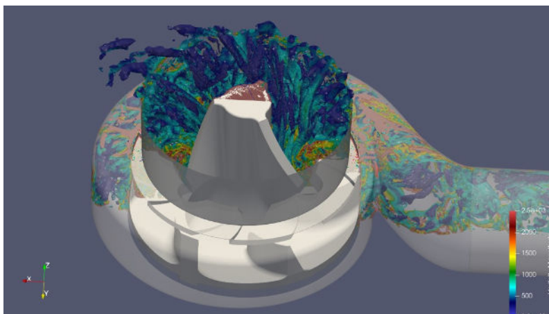
Figure-1: Full computational domain, the impeller and vortical structures inside the suction cone.
