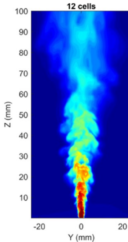
Large Eddy Simulation of hydrogen accidental release: Instantaneous Hydrogen mole fraction contours for the case of 12 cells discretization of the release diameter (contour levels are from 0 to 1).
