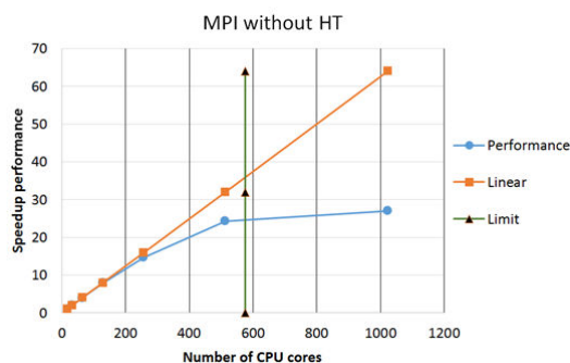
Speedup performance for modelling of a trimaran motion
