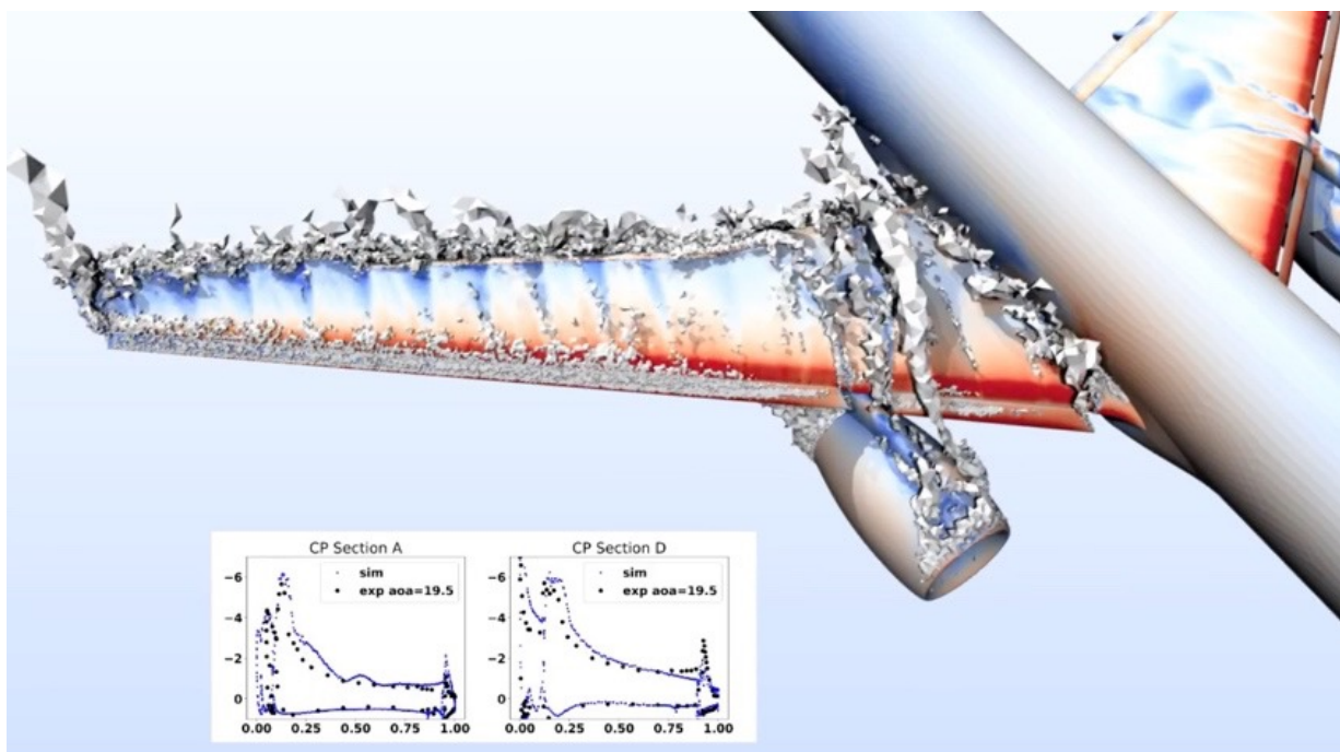
Simulation example of aircraft aerodynamics.
