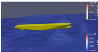
CFD simulation of the wave pattern of a ship on calm water
