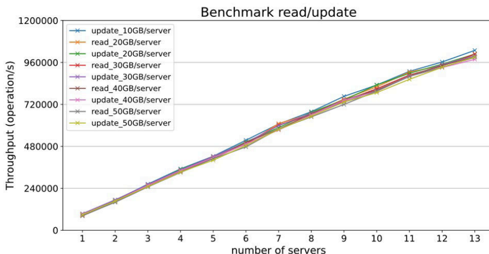
Figure 1. Linear scalability: the sensitivity of performance to table size is not significant.
