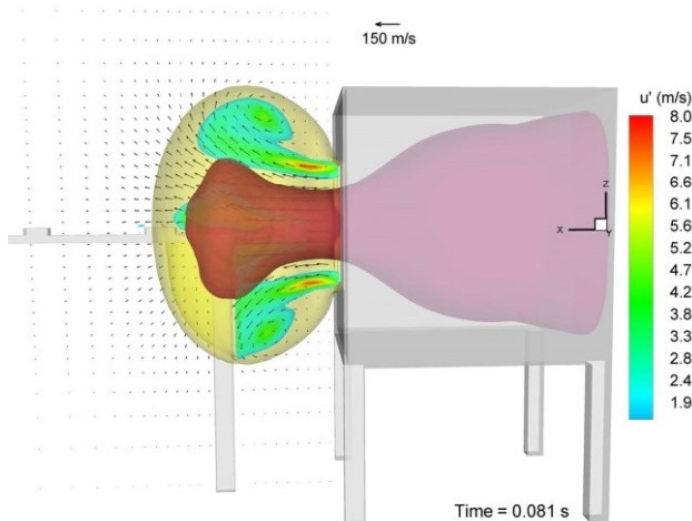
Simulation of an explosion in a vented room: Fuel mass fraction isosurface (yellow) and flame front surface (dark red) along with u' contours and velocity vectors at the onset of external explosion
