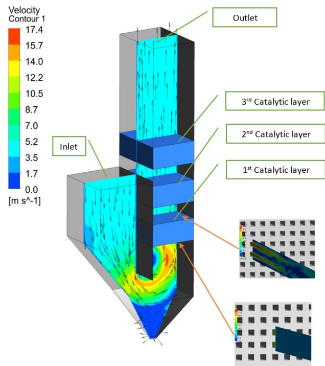
CFD simulation of SCR process
