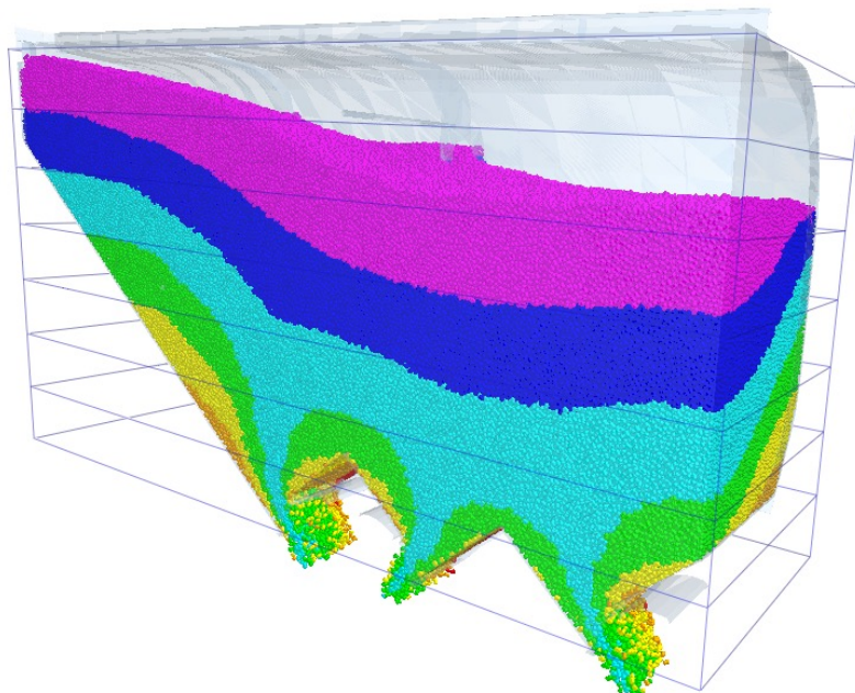
Ongoing simulation of emptying a freight wagon box – one-quarter simulation model.
