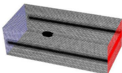
Generation of the mesh, the total number of cells 9 631 050
