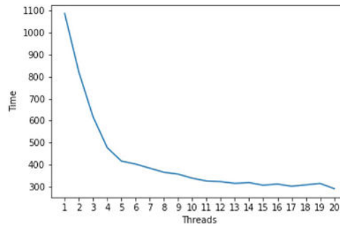
Figure 2. Execution time in seconds w.r.t number of threads used.
