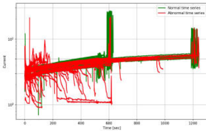
Figure 1: Time Series, normal (green), abnormal (red)
