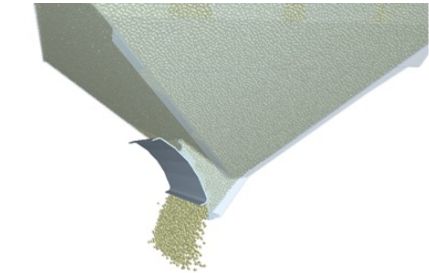
Calculations of the frictional and normal force from the flowing bulk material (grain) on the hopper closing mechanism.
