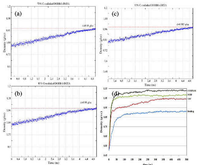
Figure 3: Equilibration of the density for crosslinked epoxy polymer with cross-linking degree (a) 70% (b) 80% (c) 90% using polymer consistent force field (PCFF) through 5 ns NPT dynamics. Each system cooled from 600 K to 298.5K (d) Equilibration of the density using different force fields through 500 ps NPT dynamics (Reference: B. Arab, A. Shokuhfar, J. Nano-Electron. Phys. 5 No 1, 01013 (2013))
