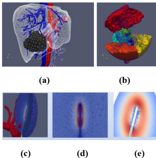
Figure 1: Radio-frequency liver ablation simulations: (a) Triangulated liver with a tumor inside via Netgen; (b) Domain decomposition via ParMETIS; (c) Visualization of the bipolar probe within the tumor; (d) The computational domain; (e) Visualization of the results: isolines on the temperature field
