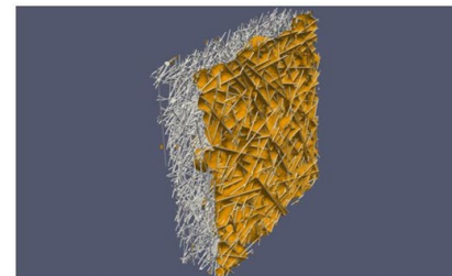
Oil interface in filter medium - inlet side
