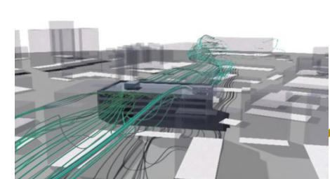
Wind path lines passing car park under planning
