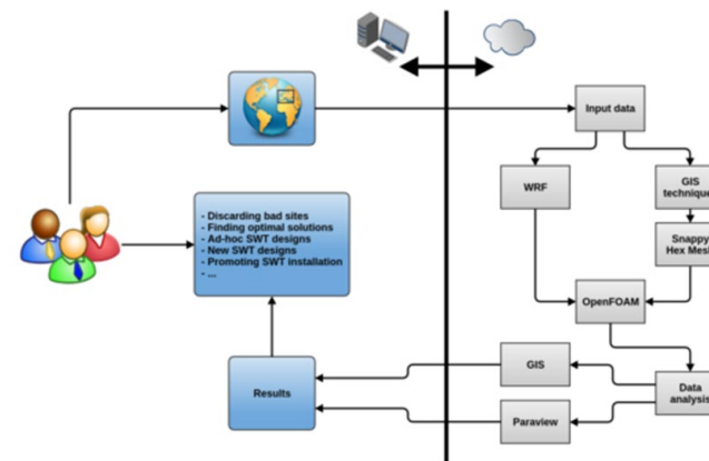
Workflow diagram representing the interaction between Cloud computing software solution and users/decision makers for wind-turbine position optimization
